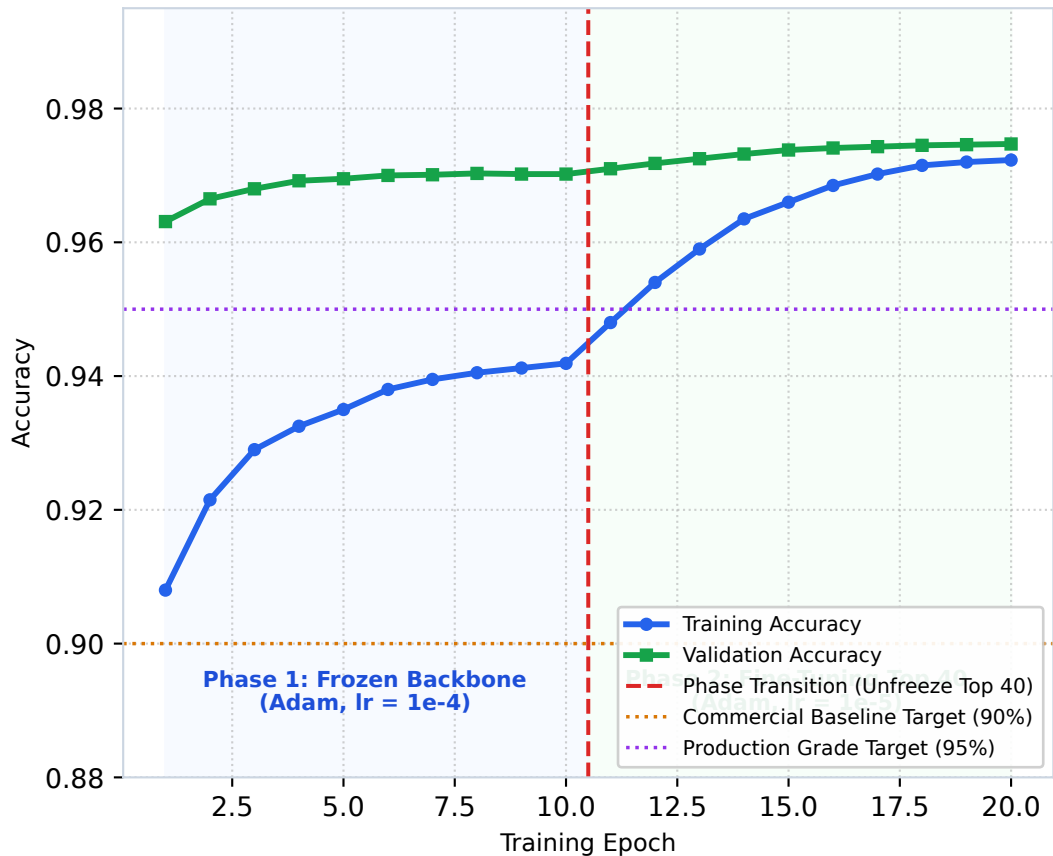
Figure 3(a): Model Classification Accuracy Across Training Epochs (Evaluating Convergence Against Commercial Thresholds)
